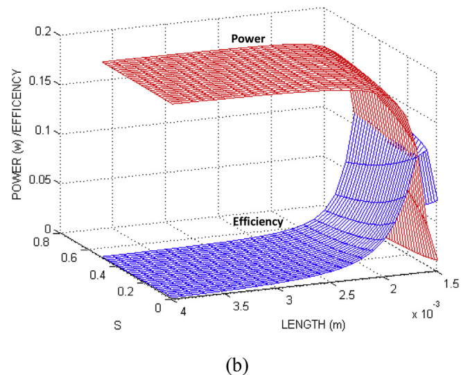
Fig. 7. 3-D view of output power and efficiency with pin length ( L ) and shape factor ( S ) for two values of temperature ratio ( \theta ): a) \theta = 0.4 and b) \theta = 0.6 .
