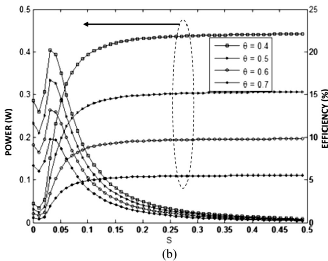
Fig. 6. Variation of thermoelectric power and efficiency with shape factor ( S ) for different values of temperature ratios: a) pin length L = 0.004 m and b) pin length L = 0.001 m.
